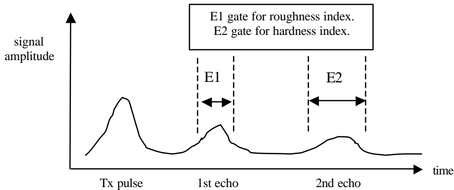
Fig. 4.11 “RoxAnn - Quantification of Roughness (E1) & Hardness (E2)”
